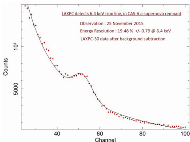
Figure 1. CasS (supernova remnant) observation of LAXPC30 showing \sim 20\% energy resolution at 6.4 keV.
