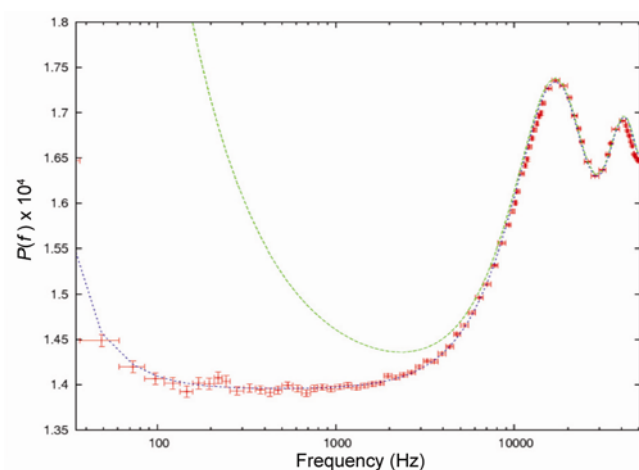
Figure 2. High-frequency rebinned power density spectrum of GRS 1915 + 105 in the steep power law class observed during 5–7 March 2016. The power spectrum matches well with the predicted Poisson noise level with a dead time of t = 42.3 \mu\text{s} and a low-frequency power-law component. The green line shows the expected peak power of a QPO with quality factor Q = 4 and rms of 5% (ref. 4).
